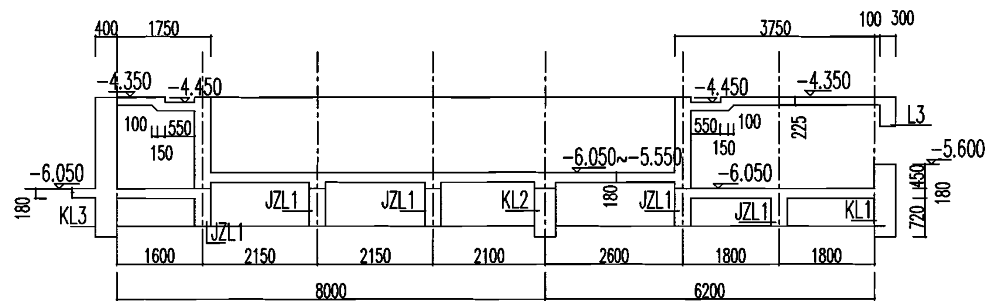
2-2
